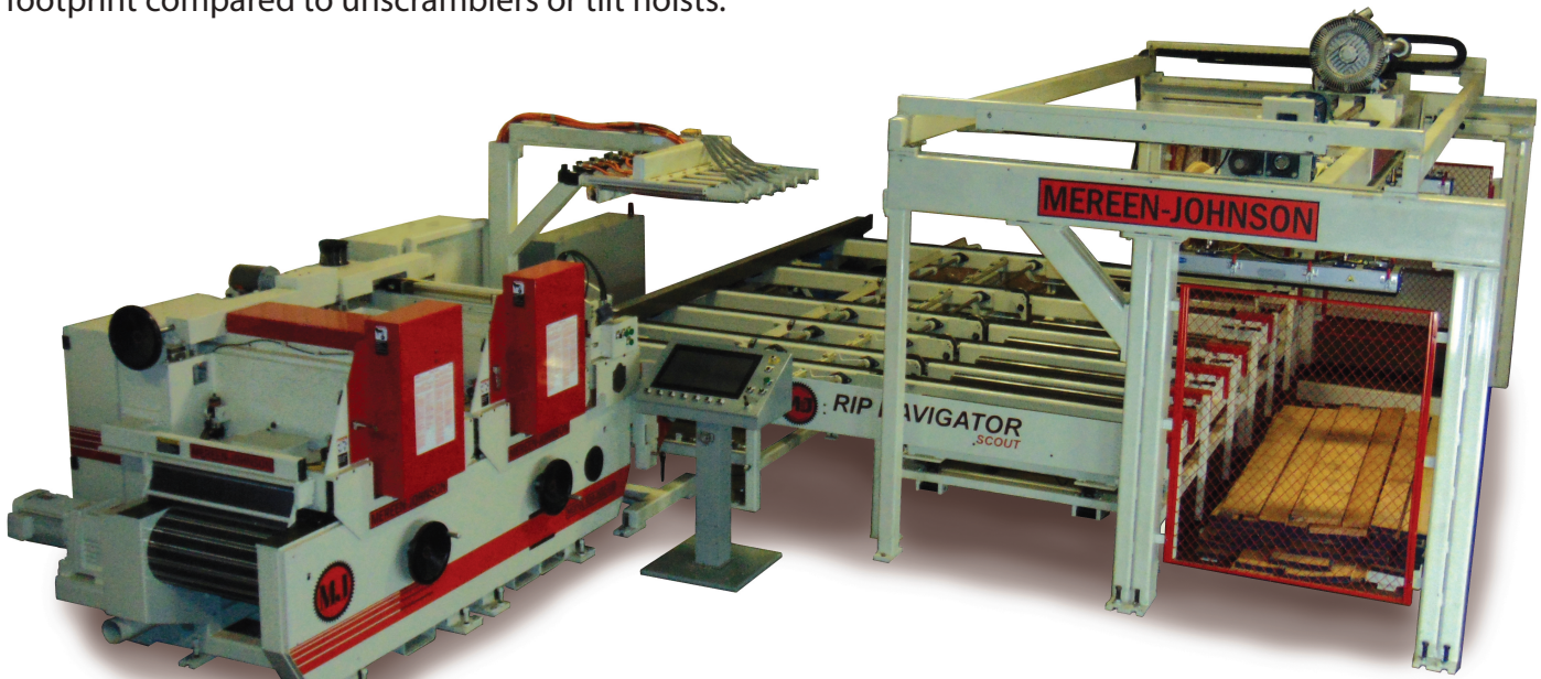
Model 524DDC/SR Edging Rip Saw with Rip Navigator Scout Optimizing System and Scout Lumber Loader
