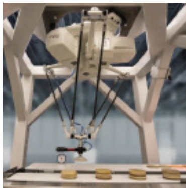
Sorting & Stacking
