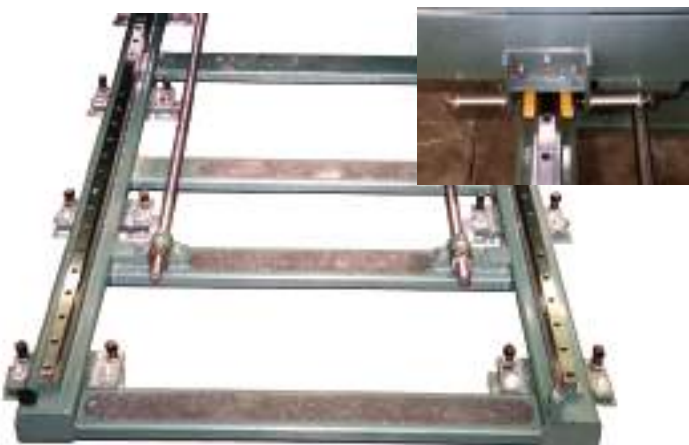
Machine Base: Heavy wall structural steel weldment with linear rails and air actuated position lock
